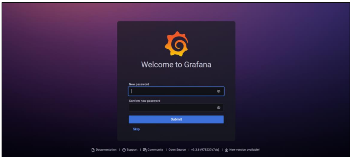
Figure 7: Grafana Login
