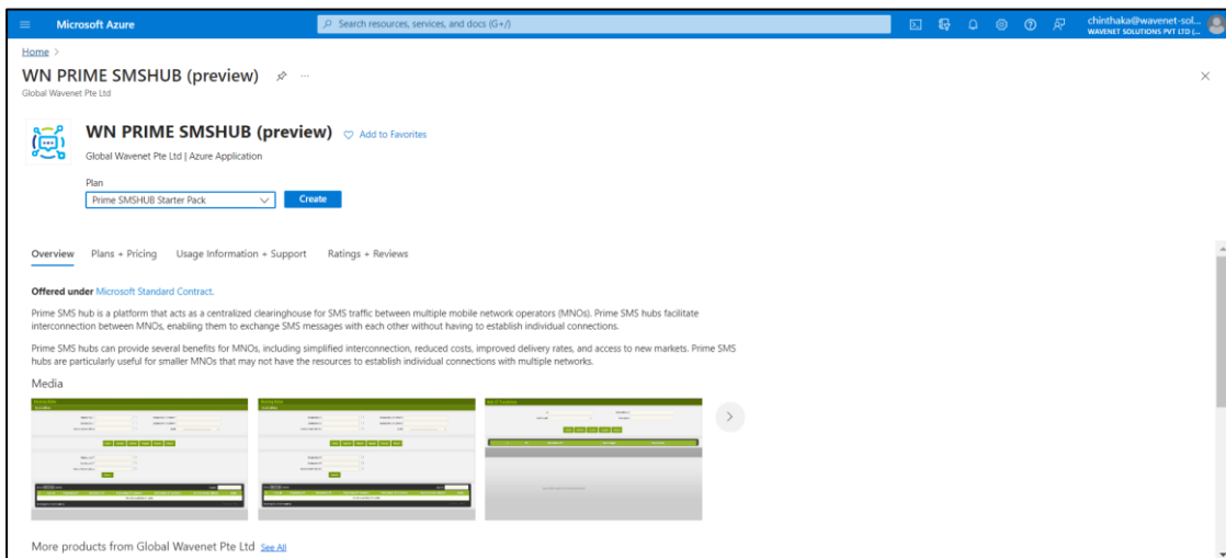
Figure 1: Selecting Service
