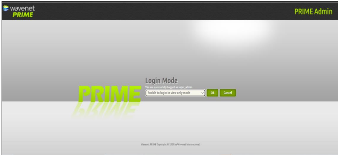
Figure 6: Prime Login
