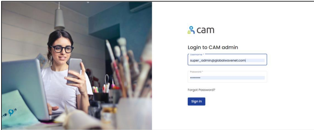
Figure 4: CAM Authentication
